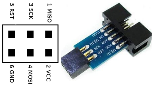
ICSP Port, Front View and 6Pins/10Pins connector.
